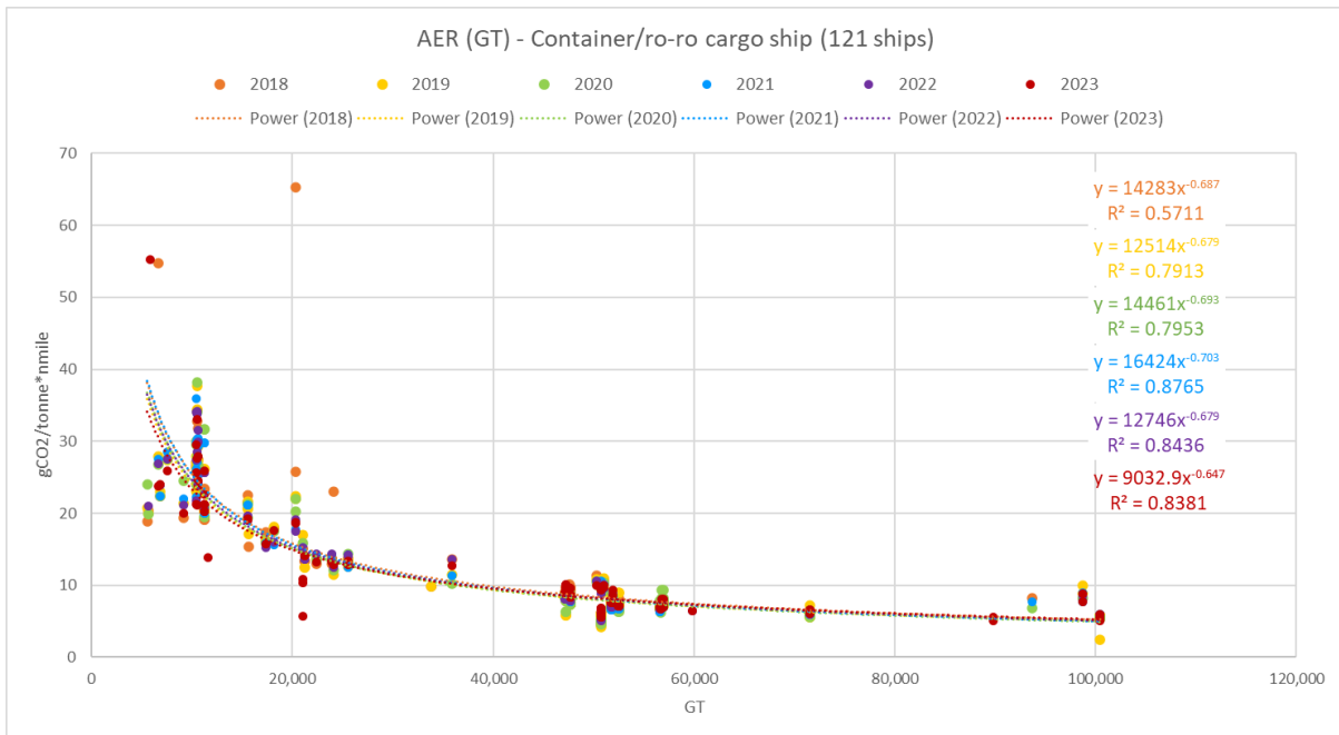
Figure 40: Plot of attained AER values of container-ro-ro cargo ships over the reporting years and associated trendlines
